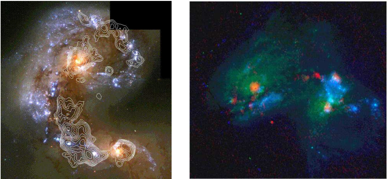
Fig. 1. Left: Composite optical (Whitmore et al. 1999) and CO (Wilson et al. 2000) image of the nearest merger, the Antennae, 2' (12 kpc) on a side. Right: Composite 250 nm (blue), 812 nm (green), and 6 cm (red) image of Arp 299, 50'' (10 kpc) on a side. Images at 250 nm and 812 nm from Alonso-Herrero et al. (2000); radio image from Neff et al. (2004).
