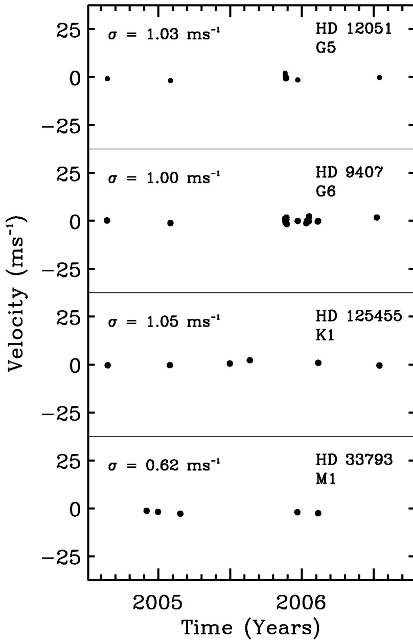
Figure 2- Some of the quietest stars on the California-Carnegie Exoplanet survey.
