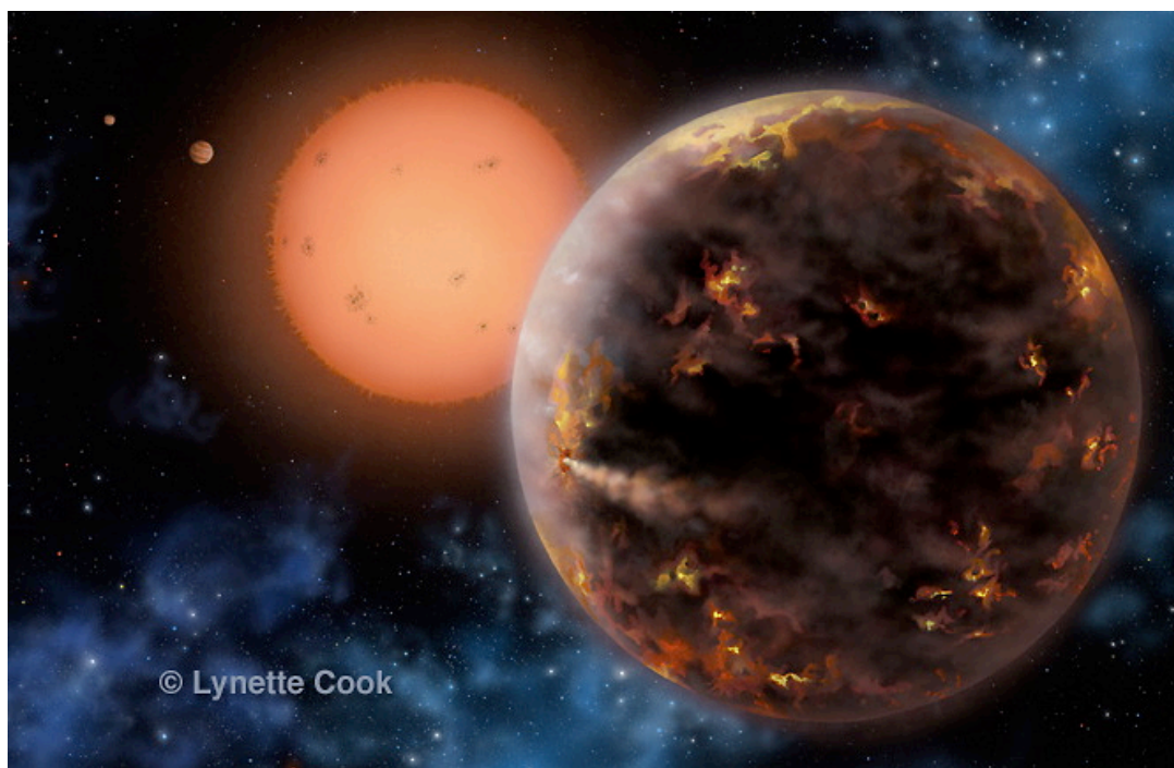
Figure 5- The remarkable triple planet system around the nearby M4 dwarf GJ 876.
