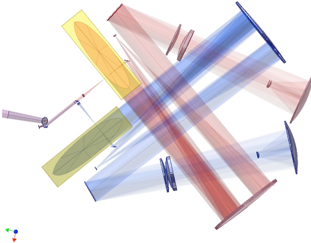
Figure 4- Top view of MTHR's high-resolution mode.
