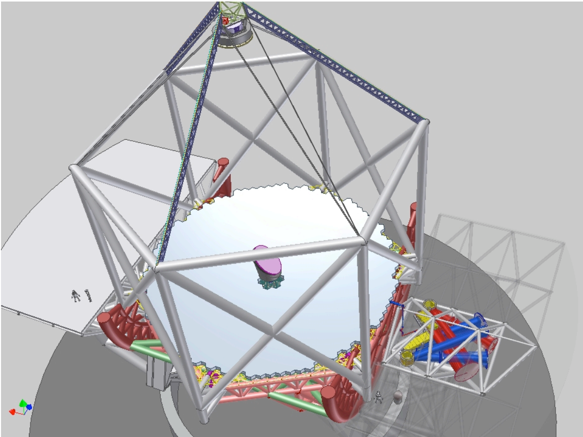
Figure 3- CAD rendering of MTHR at an f/15 focus, under the left Nasmyth platform.
