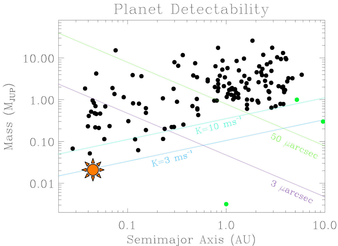
Figure 1- Planet discovery space for stars at 15 parsecs.
