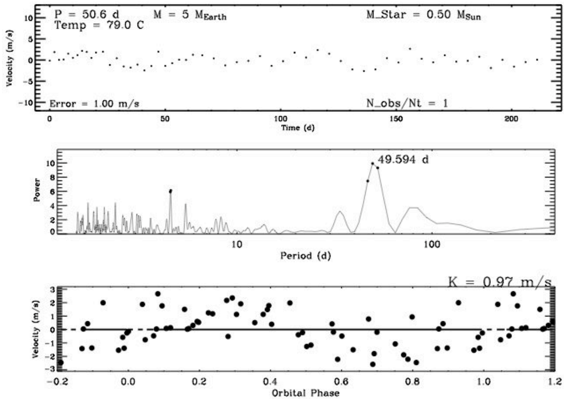
Figure 6- Detection of a 5 M_{\text{Earth}} planet in the HZ of an M2 dwarf.
