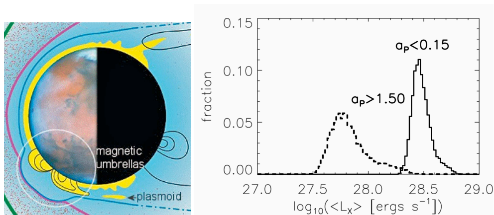
Fig. 1.— Left: Model of ablation of the Martian atmosphere involving the formation and escape of magnetic plasmoids trapping atmospheric gas (Brain 2008). Right: Mean X-ray luminosity of stars with close-in giant planets ( a_p < 0.15\text{AU} ) compared to that with extended orbits ( a_p > 1.5\text{AU} ). The close-in sample exhibits significantly higher activity levels ( a_p > 1.5 AU; Kashyap et al. 2008).
