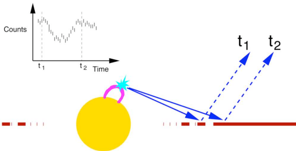
Fig. 2.— X-ray reverberation mapping of protoplanetary disks with the fluorescent Fe 6.4 keV line. Bright flares on the central star are reprocessed by the disk and this signal is revealed in spectra in the light of the cold Fe K fluorescence line. The variations of the flux from this line with time can reveal the location of gaps in the disk where planets are forming.
